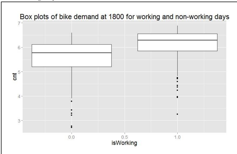
Figure 16. Box plots of bike demand at 1800 for working and nonworking days
