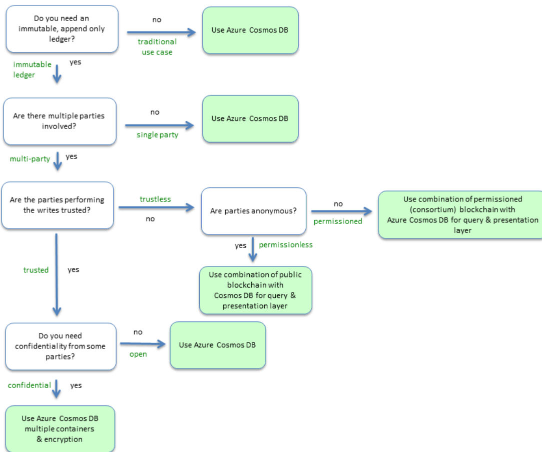
Figure 1: Blockchain workflow with Azure Cosmos DB
